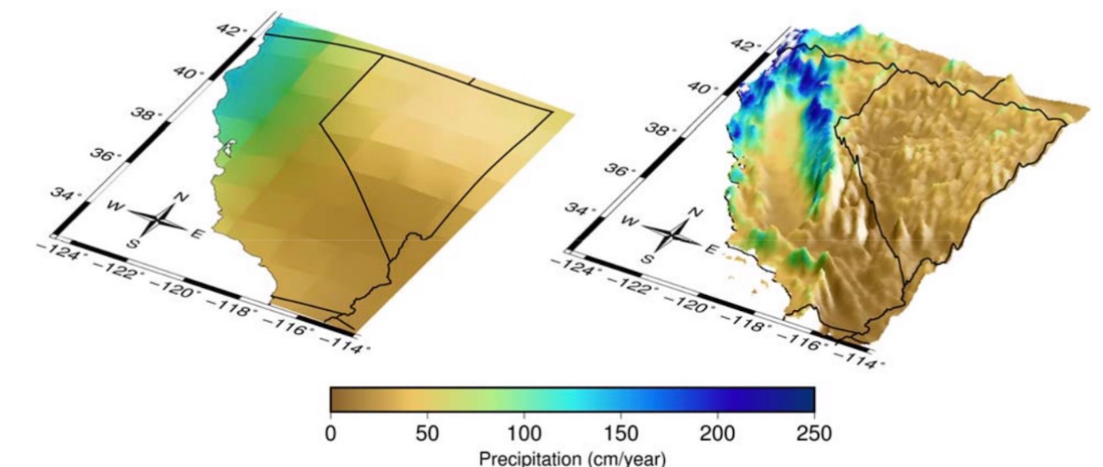
Figure 1: Resolution difference in precipitation between the raw GCM output at a coarse resolution (left) and the fine-scale LOCA2-Hybrid downscaled output (right), showcasing how the additional granularity now depicts California climate more accurately. Figure from Pierce et al. 2018 .
