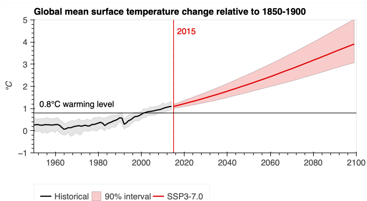
Figure 2: Estimate of the year the world reached 0.8 °C of warming. Figure produced by the Cal-Adapt: Analytics Engine (data source: IPCC ).
